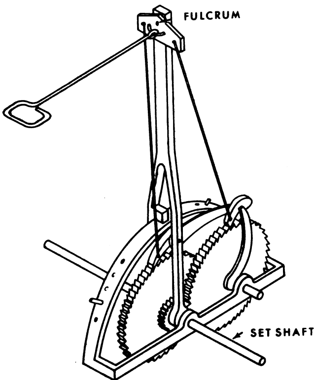
Figure 8-16. Lever-actuated networks.
